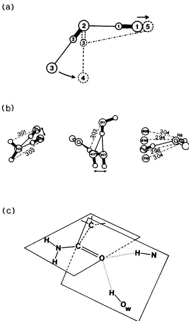
FIGURE 8 (a) The operation of the RR3 repulsive restraint in the decrease of O \cdots O \cdots O H-bond angles. As O_3 moves to O_4 , that is the O \cdots O \cdots O angle decreases, the O_1 \cdots O_2 H-bond distance has to increase ( O_1 moves to O_5 ) to maintain the minimum H_2 \cdots O_1 contact distance of \sim 3.0 Å ( O-H distances fixed to 0.8 Å). (b) H_2 \cdots O_1 contacts involved in the local disorder around the main water sites 223, 217, and 410 of networks A and B . (c) Carbonyl plane: the H-bonded deuteriums of the amide and water and the C=O atoms of the carbonyl group lie very close to a plane for the majority of carbonyl groups.
