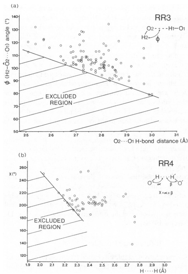
FIGURE 7 (a) Plot of H_2-O_2 \cdots O_1 angles ( \phi ) vs. O_2 \cdots O_1 H-bond distances for waters involved in hydrogen bonds within crystal hydrates (neutron structures). The solid line represents the minimum allowed values. Configurations are not found that lie significantly below this approximate cutoff line. (b) Plot of water-water H \cdots H contacts vs. \chi , the sum of the angles \alpha and \beta subtended at the hydrogen atoms (see inset motif).
